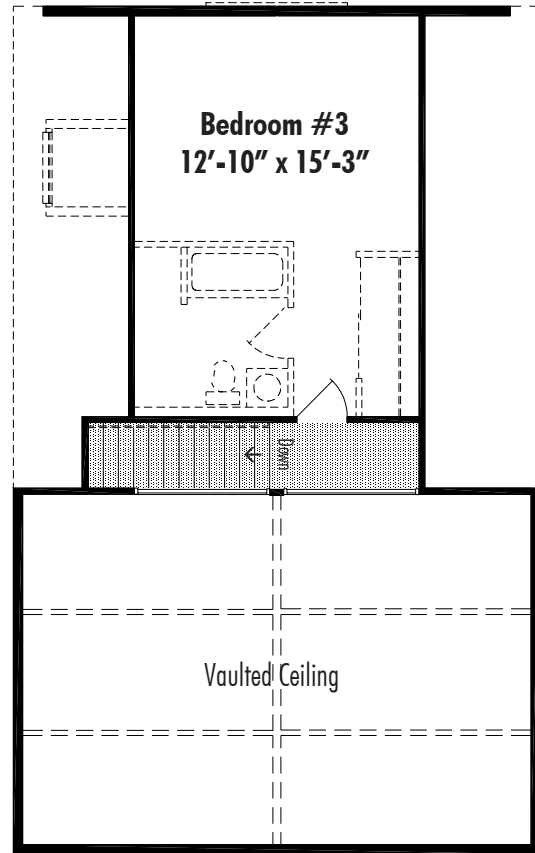
Chalet I A Second Floor
