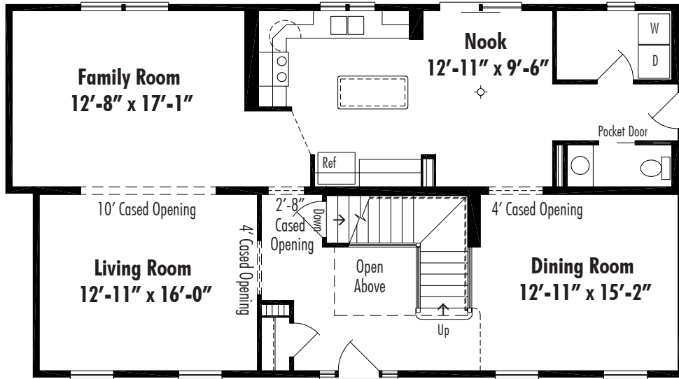
Alexandria II D Basement 27'-4" x 48/50', Total Living Area 2592 Sq. Ft.
