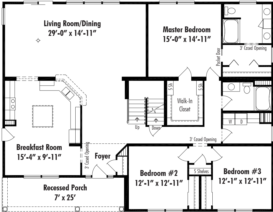
Modesto B Basement 43' x 56' 2232 Sq. Ft. Living Area
