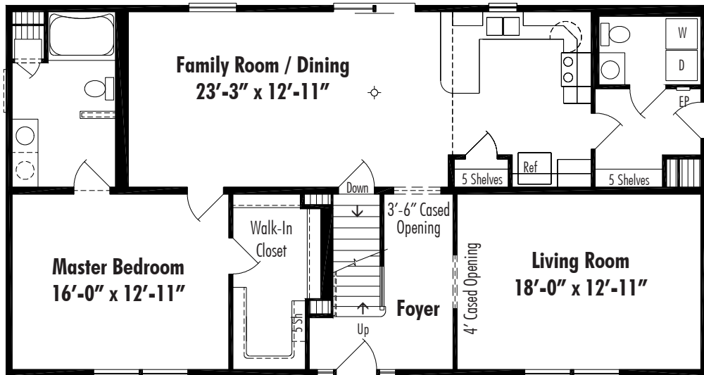
Lexington B Basement 27'-4" x 52', First Floor Living Area 1421 Sq. Ft.
