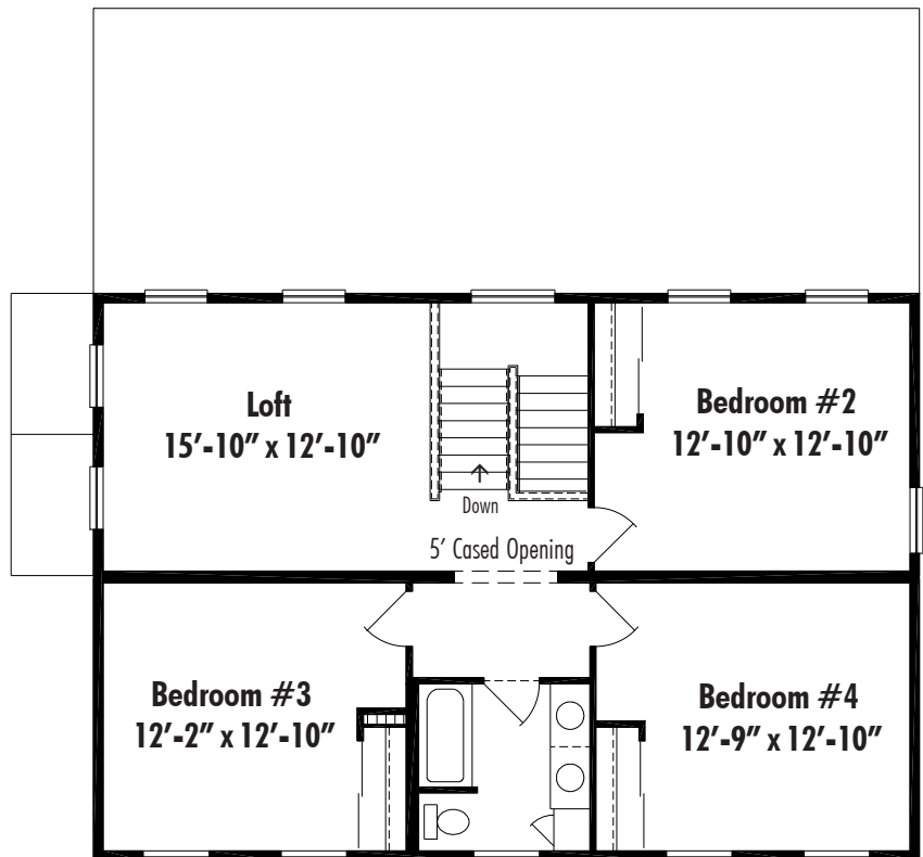
Worthington Second Floor
