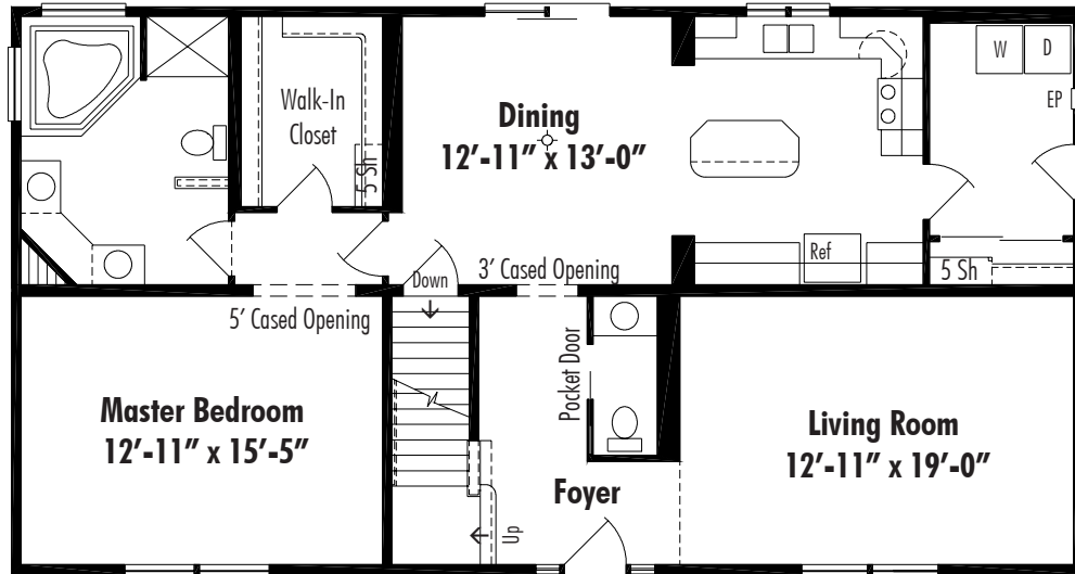
Monticello III F Basement 27'-4" x 52', Total Living Area 2325 Sq. Ft.
