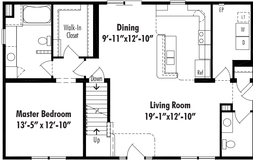
Jefferson I B Basement 27'-4" x 44' 2 / 30 ' 2035 Sq. Ft. Total Living Area
